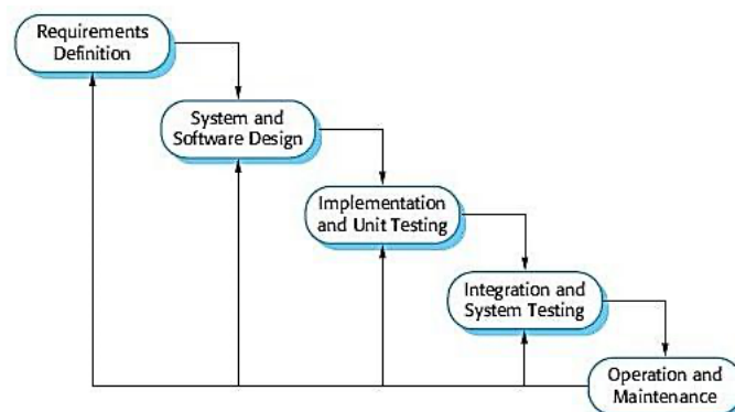
Gambar 2. Model Waterfall
